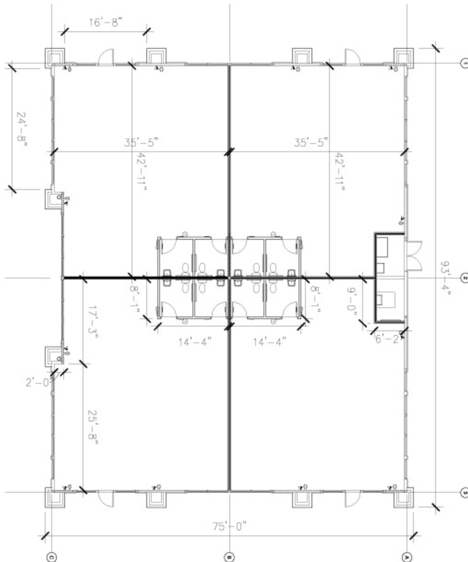
Type 2 Floor Plan
